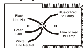
Wiring Diagram for Stud Models
