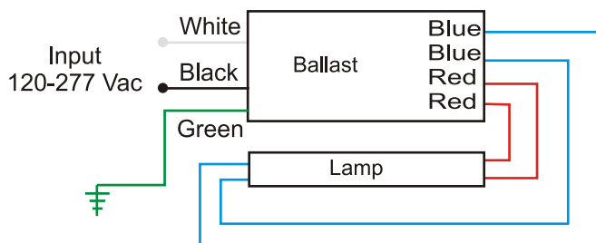
Ballast Wiring Diagram
